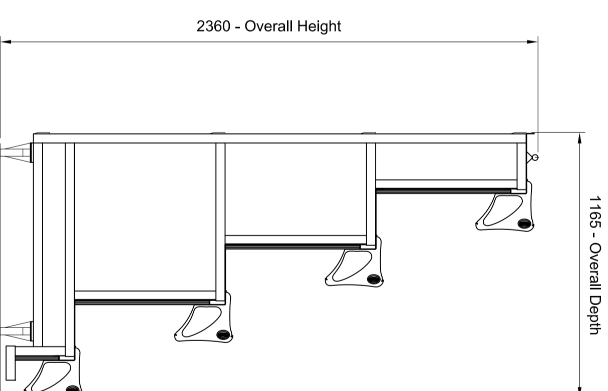
SIDE ELEVATION (Unit in Store Position)
